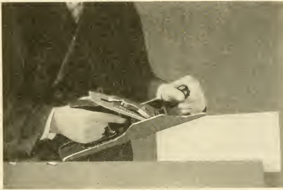
Fig. 17. Holding the Plane at an Angle to Cut a Chamfer
